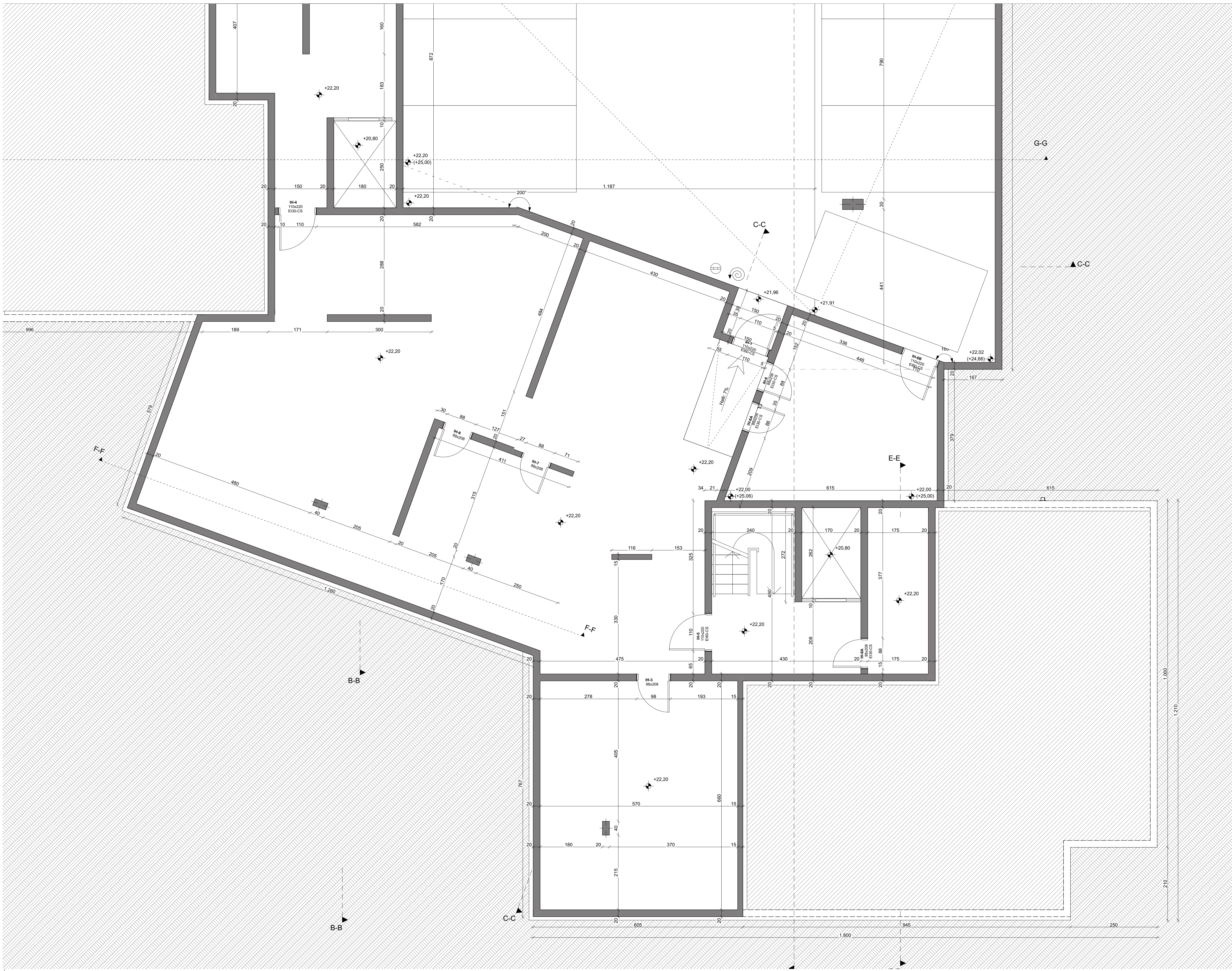
0. kjallari
